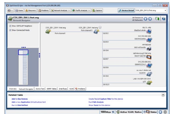
Network Navigator
